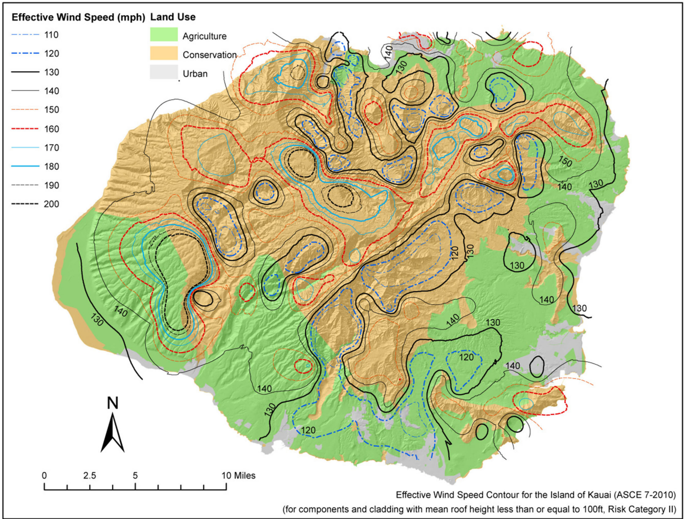
Figure 1609.3.2.2(f) County of Kauai Effective Ultimate Wind Speed, V_{eff-ult} , for Components and Cladding for Risk Category II Buildings less than 100 feet Tall
