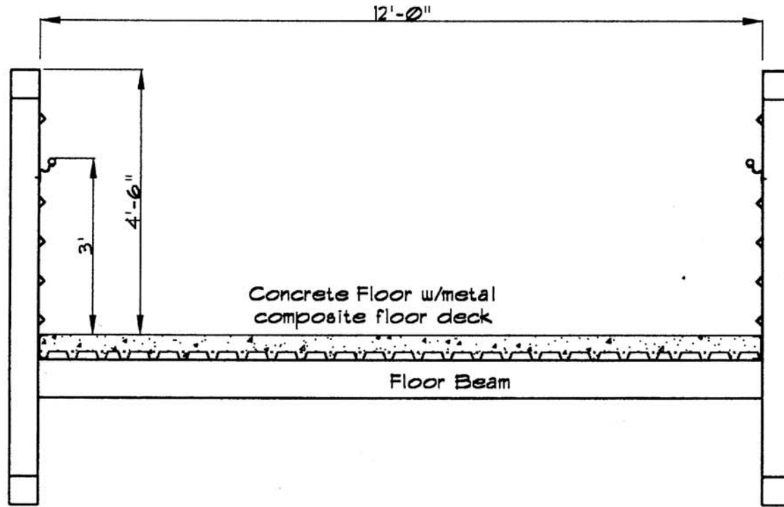
Typical Bridge Section
